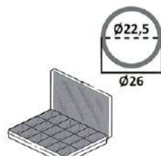
15141 Shim Kit \varnothing 26 - Hole \varnothing 22,5 Total items 470 pcs. — 54 shims size from 2,04 to 2,50 (cut 0,01)
