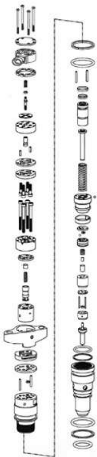
CATERPILLAR® C7/C9
